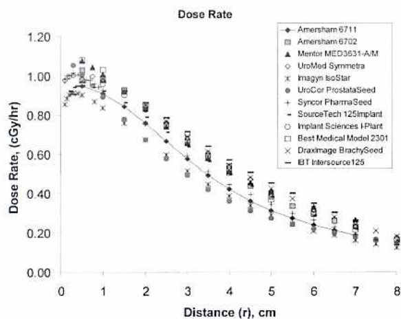
FIG. 5. Dose Rate Values for source strength of 1 U.
