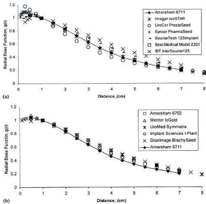
FIG. 3. Radial Dose Function g(r) : (a) Radial Dose Functions for the sources with the radioactivity adsorbed onto the internal core of the source, (b) Radial Dose Functions for the sources with the radioactivity adsorbed onto the internal core of the source.
