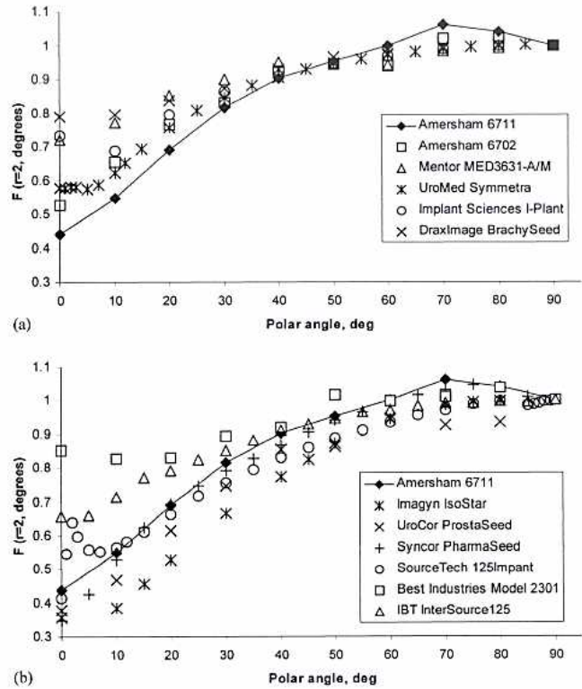
FIG. 4. Anisotropy Function F(r, \theta) : (a) Anisotropy Functions for the sources with the radioactivity adsorbed onto the internal core of the source for a radius of 2 cm, (b) Anisotropy Functions for the sources with the radioactivity adsorbed onto the internal core of the source for a radius of 2 cm.
