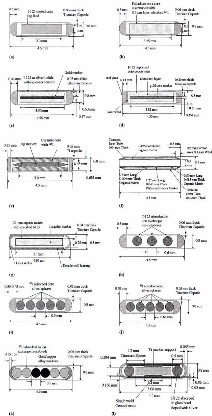
FIG. 1. Cross-Sectional drawings of sources with a Rod, Wire, or Cylinder internal core design; (a) Amersham 6711 OncoSeed, (b) Syncor PharmaSeed, (c) UroMed Symmetra, (d) SourceTech Medical ^{125}\text{I} Implant, (e) Med-Tec I-Plant, (f) International Brachytherapy, Inc. InterSource ^{125}\text{I} , (g) Best Medical Model 2301 (h) Amersham 6702, (i) UroCor ProstaSeed, (j) Imagyn IsoSTAR, (k) Mentor's IoGold, (l) DraxImage BrachySeed.
